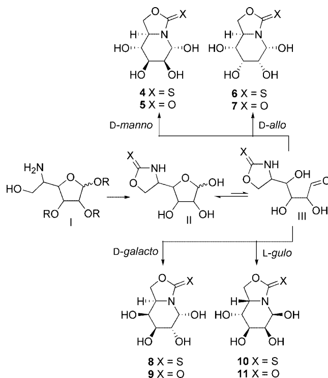
Figure 2. Synthetic strategy for the preparation of the reducing (+)-2-oxacastanospermine diastereomers from 5,6-cyclic (thio)carbamate hexofuranoses (II), obtained from 5-amino-5-deoxysugar precursors (I), via the open-chain aldehyde form (III).
