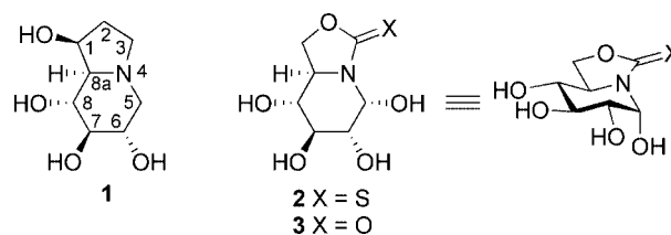
Figure 1. Structures of (+)-castanospermine and of the reducing thiocarbamic and carbamic analogues.
