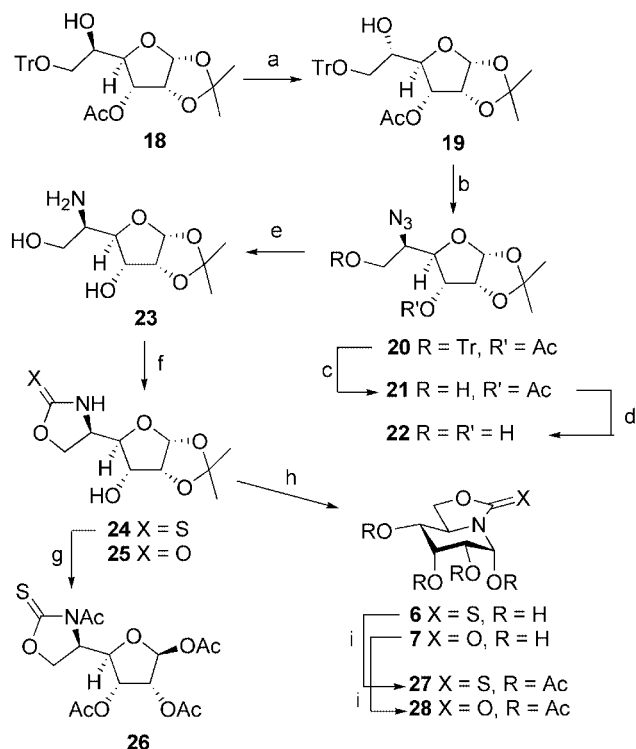
Scheme 2. Reagents and conditions: a, 1. \text{TiF}_2\text{O} , \text{CH}_2\text{Cl}_2 , pyridine, -25^\circ\text{C} \rightarrow room temp., 30 min; 2. \text{NaNO}_2 , DMF, room temp., 18 h, 51%; b, 1. \text{TiF}_2\text{O} , \text{CH}_2\text{Cl}_2 , pyridine, -25^\circ\text{C} \rightarrow room temp., 30 min; 2. \text{NaN}_3 , DMF, room temp., 18 h, 85%; c, \text{BF}_3\text{-Et}_2\text{O} , MeOH, 0^\circ\text{C} \rightarrow room temp., 2 h, 80%; d, NaOMe, MeOH, 85%; e, \text{H}_2 , Pd/C, MeOH, room temp., 1 h, quant.; f, for 24 : \text{CS}_2 , DCC, \text{CH}_2\text{Cl}_2 , -10^\circ\text{C} \rightarrow room temp., 5 h, 89%; for 25 : triphosgene, DIPEA, \text{CH}_2\text{Cl}_2 , 0^\circ\text{C} \rightarrow room temp., 20 min, 89%; g, 1.90% TFA/water, 0^\circ\text{C} , 15 min; 2. \text{Ac}_2\text{O} /pyridine; h, 1. 90% TFA/water, 0^\circ\text{C} , 15 min; 2. \text{Ac}_2\text{O} /pyridine; 3. NaOMe, MeOH, 50–64%; i, \text{Ac}_2\text{O} /pyridine, 98%.
