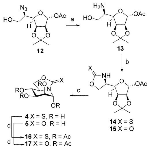
Scheme 1. Reagents and conditions: a, H_2 , Pd/C, MeOH, room temp., 2 h, quant.; b, for 14 : CS_2 , DCC, CH_2Cl_2 , -10^\circ C \rightarrow room temp., 2.5 h, 78%; for 15 : triphosgene, DIPEA, CH_2Cl_2 , 0^\circ C \rightarrow room temp., 15 min, 65%; c, 1. NaOMe, MeOH; 2. 90% TFA/water, 0^\circ C , 15 min, 74–82%; d, Ac_2O /pyridine, 95–98%.
