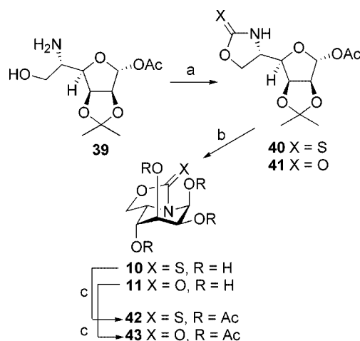
Scheme 4. Reagents and conditions: a, for 40: \text{CS}_2 , DCC, \text{CH}_2\text{Cl}_2 , -10^\circ\text{C} \rightarrow \text{room temp.} , 8 h, 70%; for 41: triphosgene, DIPEA, \text{CH}_2\text{Cl}_2 , 0^\circ\text{C} \rightarrow \text{room temp.} , 45 min, 43%; b, 1. 90% TFA/water, 0^\circ\text{C} , 15 min; 2. \text{Ac}_2\text{O} /pyridine; 3. NaOMe, MeOH, 50%; c, \text{Ac}_2\text{O} /pyridine, 87–90%.
