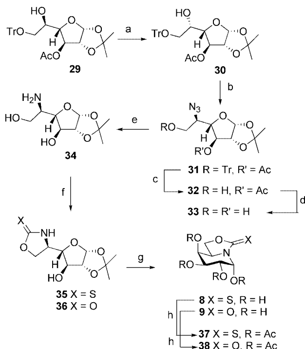
Scheme 3. Reagents and conditions: a, 1. \text{TiF}_4 , \text{CH}_2\text{Cl}_2 , pyridine, -25^\circ\text{C} \rightarrow \text{room temp.} , 30 min; 2. \text{NaNO}_2 , DMF, room temp., 24 h, 51%; b, 1. \text{TiF}_4 , \text{CH}_2\text{Cl}_2 , pyridine, -25^\circ\text{C} \rightarrow \text{room temp.} , 30 min; 2. \text{NaN}_3 , DMF, room temp., 24 h, 51%; c, \text{BF}_3 \cdot \text{Et}_2\text{O} , MeOH, 0^\circ\text{C} \rightarrow \text{room temp.} , 2 h, 75%; d, NaOMe, MeOH, 80%; e, \text{H}_2 , Pd/C, MeOH, room temp., 1 h, 96%; f, for 35: \text{CS}_2 , DCC, \text{CH}_2\text{Cl}_2 , -10^\circ\text{C} \rightarrow \text{room temp.} , 6 h, 86%; for 36: triphosgene, DIPEA, \text{CH}_2\text{Cl}_2 , 0^\circ\text{C} \rightarrow \text{room temp.} , 10 min, 90%; g, 1. 90% TFA/water, 0^\circ\text{C} , 15 min; 2. \text{Ac}_2\text{O} /pyridine; 3. NaOMe, MeOH, 65–89%; h, \text{Ac}_2\text{O} /pyridine, 82–85%.
